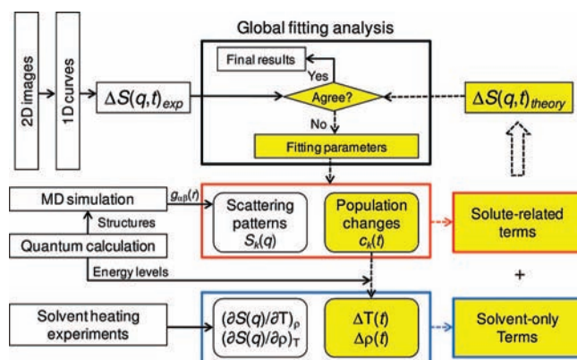
FIGURE 2. Schematic of the data analysis. The discrepancy between the theory and experiment is minimized using a global fitting analysis by considering data at all positive time delays simultaneously. Boxes with red and blue frames represent solute-related and solvent-only terms, respectively. Boxes with yellow background are involved in a typical iterative minimization procedure. See the text for details.
